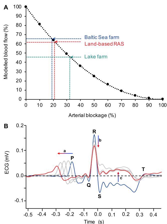
Fig. 6. The consequences of coronary obstruction on the blood flow and electrocardiogram of rainbow trout. According to Poiseuille's law, the black dashed line in (A) represents the theoretical reductions in laminar blood flow through a capillary caused by reductions in the radius of the vessel (e.g. via blockages) when assuming equal blood pressure, viscosity and capillary length. Coloured dashed lines indicate estimations of reduced coronary blood flow caused by arteriosclerotic lesions in rainbow trout from the open cage Baltic Sea farm (blue), open cage lake farm (green) and land-based RAS (red). (B) A subjectively healthy electrocardiogram (ECG) of a rainbow trout directly prior to the occlusion of the coronary artery (blue line). The ECG consists of the P-wave (atrial depolarization), the QRS-complex (ventricular depolarization) and the T-wave (ventricular repolarization). During a 30 min occlusion (from blue to red ECG trace), the time between the P-wave and R-wave increases (see a), the amplitude of the R-wave is gradually reduced (see b) and the ST-segment is elevated (see c). Grey lines in (B) represents ECG's at regular time periods throughout the occlusion period (~ every 7 min) and the black dashed line in (B) represents the isoelectric line. (For interpretation of the references to colour in this figure legend, the reader is referred to the web version of this article.)
